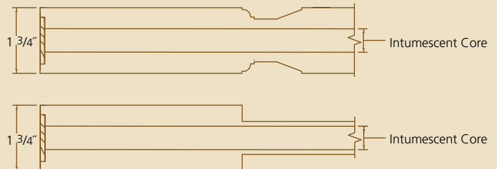
Woodgrain 90 Minute Fire Rated MDF Door
